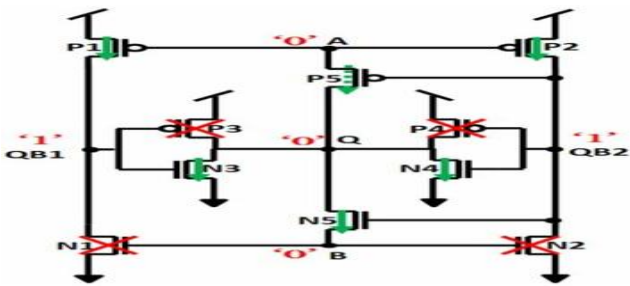
Fig. 2. Logic '0' State
